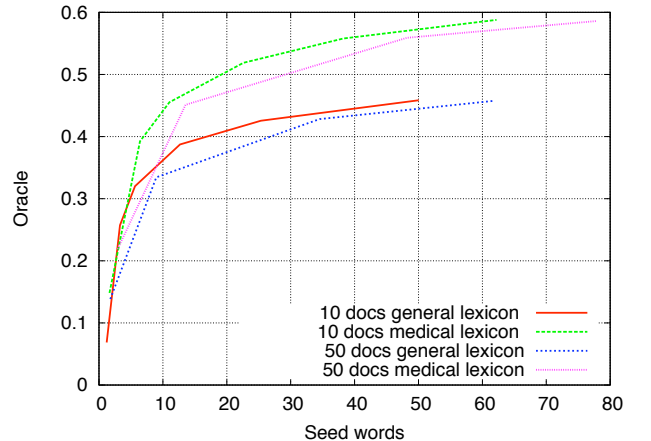
Fig. 3: Oracle score by lexicon type.
