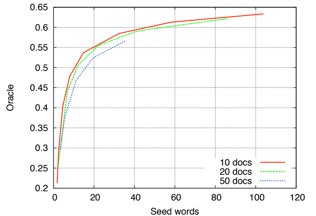
Fig. 2: Oracle score with seed word variations.
